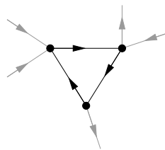
A cycle in a directed network.
