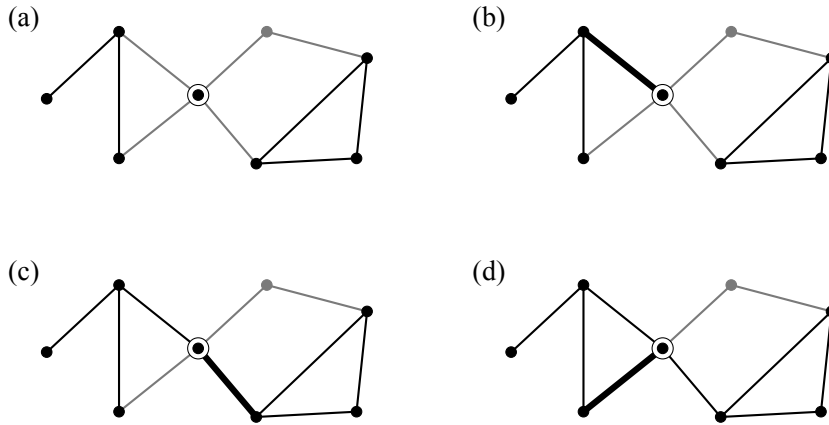
Figure 16.8: Percolation algorithm. In the percolation algorithm described in the text we add vertices to our network one by one, rather than taking them away. Each addition consists of several steps. (a) We add the vertex itself but none of its accompanying edges yet. At this stage the vertex constitutes a new cluster in its own right. (b) We start adding the accompanying edges (if any) in any order we like. Only edges that connect to other vertices already present in the network are added. The first edge added (if any are added) will thus, by definition, always join the new vertex to one of the previously existing clusters. Or to put it another way, it will join two clusters together, one of the old clusters and the new cluster that consists of just the single added vertex. (c) In this example the next edge added also joins two clusters together. (d) The final edge added joins two vertices that are already members of the same cluster, so the cluster structure of the network does not change.
