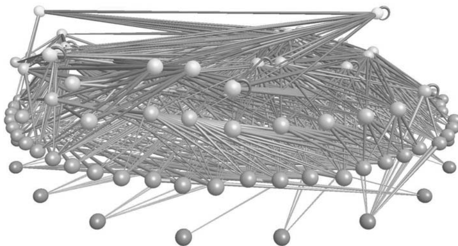
Figure 1.3: The food web of Little Rock Lake, Wisconsin. (See Plate II for color version.) This elegant picture summarizes the known predatory interactions between species in a freshwater lake in the northern United States. The vertices represent the species and the edges run between predator–prey species pairs. The vertical position of the vertices represents, roughly speaking, the trophic level of the corresponding species. The figure was created by Richard Williams and Neo Martinez [209].
