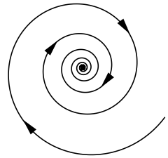
The flows around a fixed point whose Jacobian matrix has complex eigenvalues describe a spiral.
