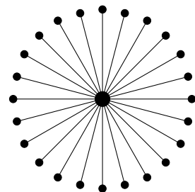
A star graph of 25 vertices.
