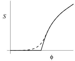
The phase transition at which the giant cluster appears is only sharp in an infinite system (solid line). In a finite sized system it gets rounded off (dashed line).
