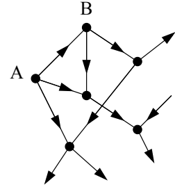
Figure 7.1: A portion of a directed network. Vertex A in this network has only outgoing edges and hence will have eigenvector centrality zero. Vertex B has outgoing edges and one incoming edge, but the ingoing one originates at A, and hence vertex B will also have centrality zero.
