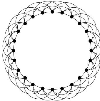
Figure 15.2: A simple one-dimensional network model. (a) Vertices are arranged on a line and each is connected to its c nearest neighbors, where c = 6 in this example. (b) The same network with periodic boundary conditions applied, making the line into a circle.
