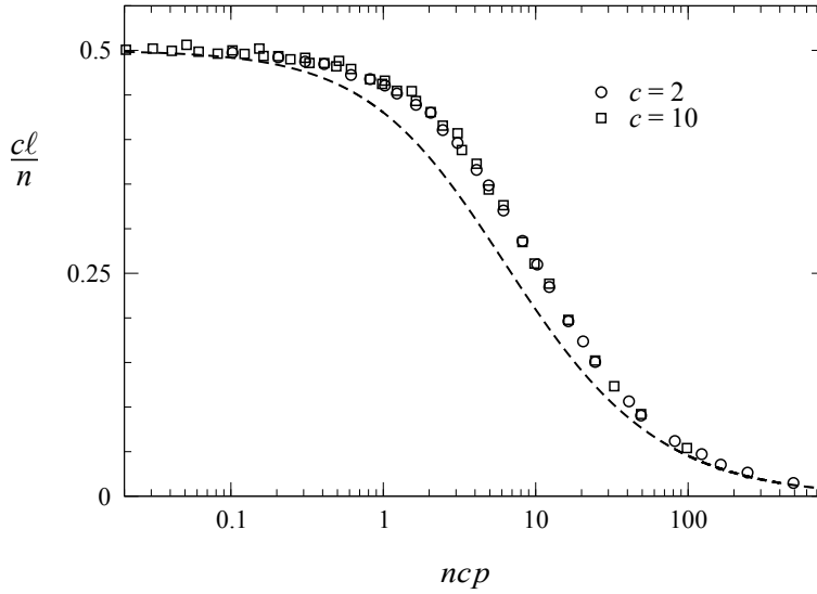
Figure 15.6: Scaling function for the small-world model. The points show numerical results for c\ell/n as a function of ncp for the small-world model with a range of parameter values n = 128 to 32\,768 and p = 1 \times 10^{-6} to 3 \times 10^{-2} , and two different values of c as marked. Each point is averaged over 1000 networks with the same parameter values. The points collapse, to a reasonable approximation, onto a single scaling function f(ncp) in agreement with Eq. (15.13). The dashed curve is the mean-field approximation to the scaling function given in Eq. (15.14).
