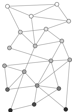
A sketch of stratified network in which most connections run between vertices at or near the same “level” in the network, with level along the vertical axis in this case and also denoted by the shades of the vertices.
