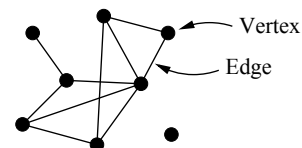
A small network composed of eight vertices and ten edges.
