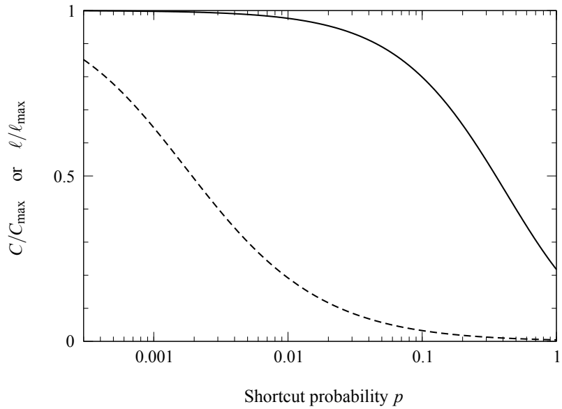
Figure 15.5: Clustering coefficient and average path length in the small-world model.
