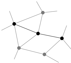
A geodesic path of length two between two vertices.
