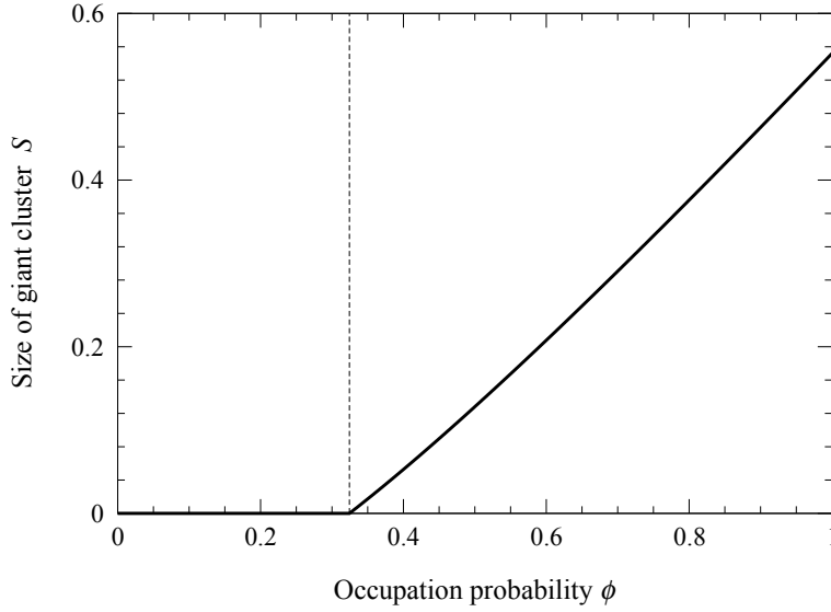
Figure 16.4: Size of the giant cluster for site percolation in the configuration model.
