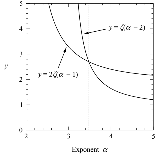
Figure 13.8: Graphical solution of Eq. (13.138). The configuration model with a pure power-law degree distribution (Eq. (13.133)) has a giant component if \zeta(\alpha-2) > 2\zeta(\alpha-1) . This happens for values of \alpha below the crossing point of the two curves.
