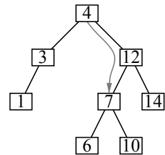
The path taken through our binary tree to locate the number 7.
