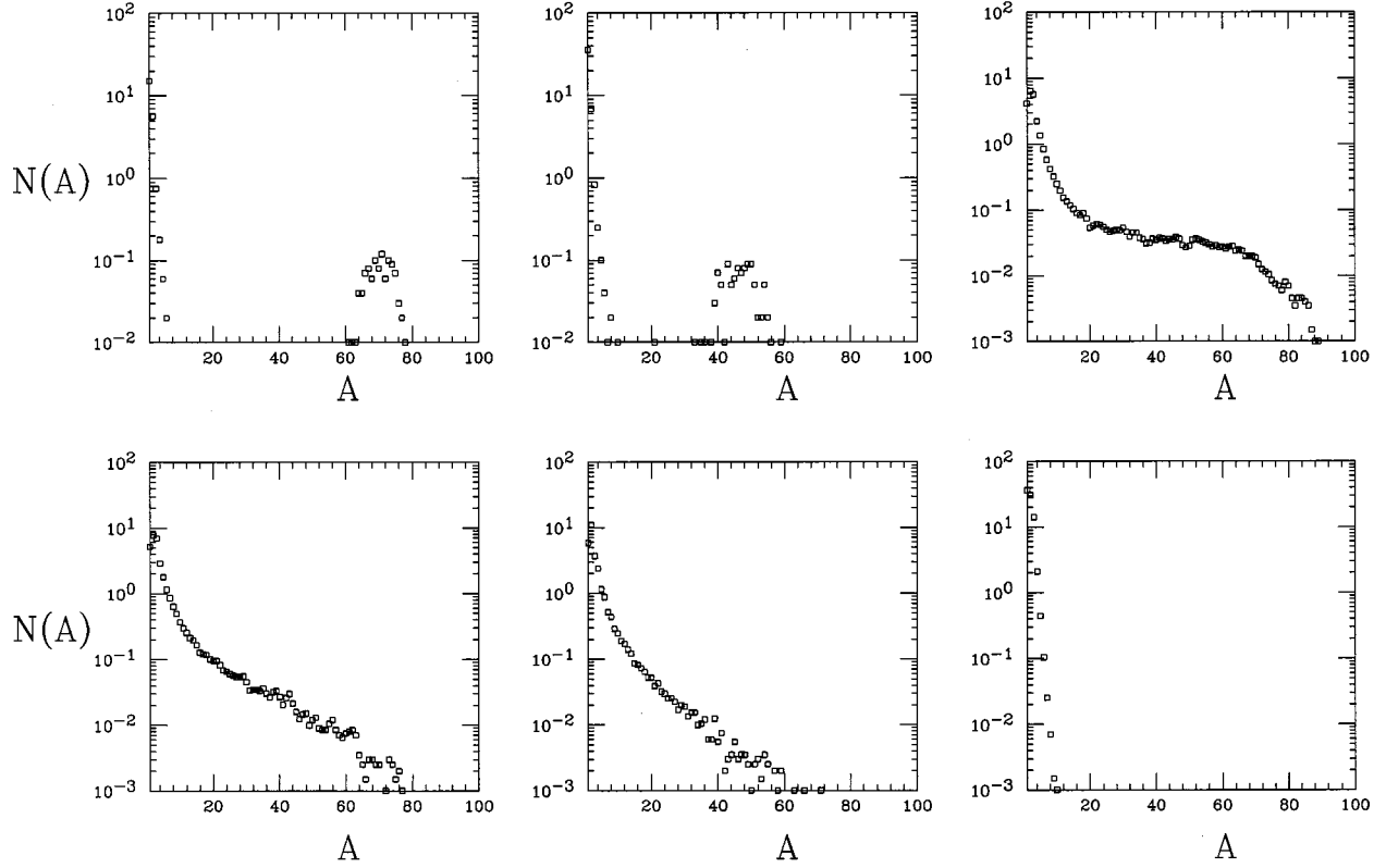
FIG. 1. Mass distributions obtained in the expansion of the system A = 100 with six different initial energies, namely, 2, 3, 4, 5, 7, and 15 MeV g from 2 to 15 MeV (beginning at the upper left corner).
