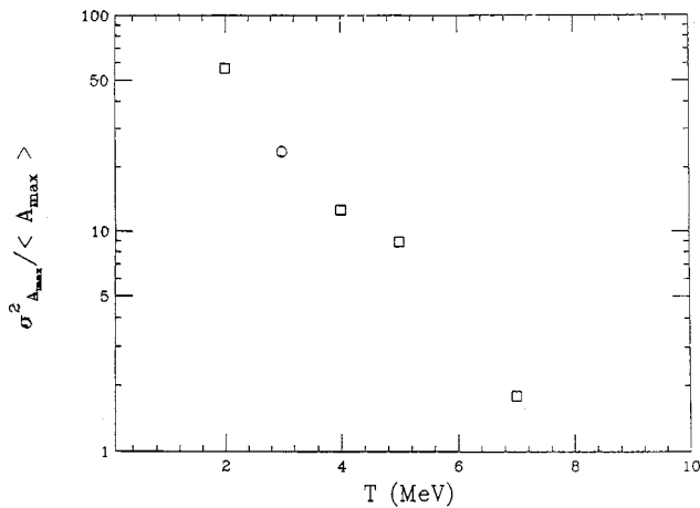
FIG. 3. Normalized variance for the random partition model when the partition is performed according to Fisher's law and the parameters are those displayed in Table I. The point for T=3 \text{ MeV} (open circle) is generated imposing the extra condition that the mass of the biggest fragment should be smaller than 60 (see text for details).
