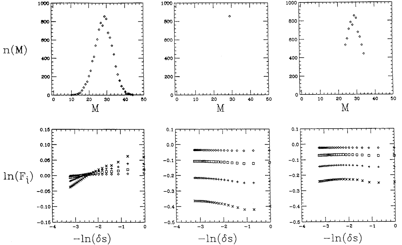
FIG. 7. In the upper panels we show the multiplicity distributions for the expansion of the system A = 100 when different ranges of multiplicities are chosen and in the lower panels the corresponding intermimty signal at T = 5 MeV. Left part: the multiplicity and intermimty when the complete set of 10 000 events is considered. Central part: in the upper panel we show the effect of retaining just one multiplicity (the most probable one) that involves 748 events; in the lower panel we see that the intermimty signal is gone. In the right panels we show the effect on the IS of using only the central events of the multiplicity distribution.
