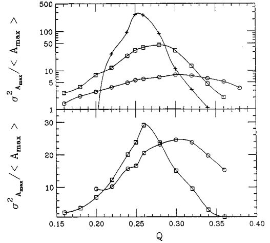
FIG. 4. Normalized variance for bond percolation in finite systems as a function of the bond activation probability Q , for, in the upper part, lattices of sizes 20 \times 20 \times 20 (crosses), 10 \times 10 \times 10 (squares), and 5 \times 5 \times 5 (circles) with unrestricted multiplicity. It is readily seen that the smaller is the size of the lattice the bigger is the difference of the maximum of the curves from the percolation critical bond for infinite lattice ( Q_c=0.23 ). This is a clear manifestation of finite size effects. The lower part shows the same as the upper part but for fixed multiplicity and for lattices of sizes 10 \times 10 \times 10 (squares) and 5 \times 5 \times 5 (circles).
