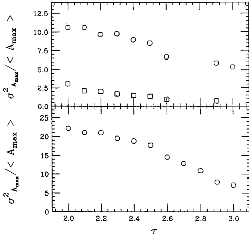
FIG. 2. Normalized variance for the random partition model when the partitioning is performed according to a power law with \tau in the range 2 < \tau < 3 (the physically interesting region) for, in the upper part, the system with A_{tot}=100 with unrestricted multiplicity (open squares) and fixed multiplicity (in the most probable value, open circles), and in the lower part the same but for A_{tot}=200 and free multiplicity. In all cases no signal is observed.
