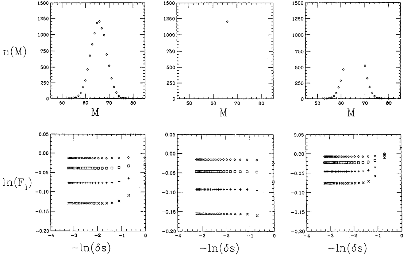
FIG. 9. Same as Fig. 7 but for the T=15 MeV case.
