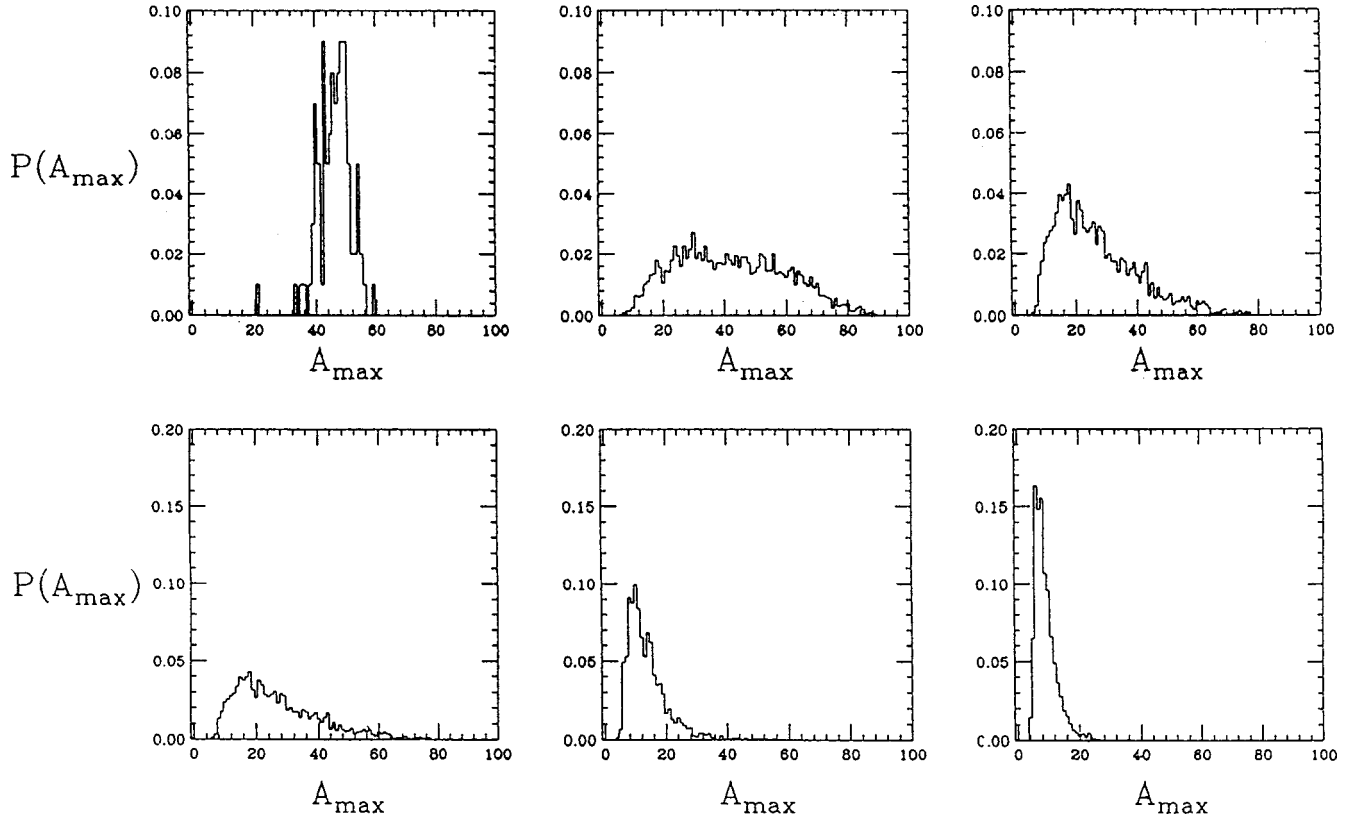
FIG. 5. We show the probability distribution of the size of the maximum fragment for six different initial temperatures for the A = 100 fragmenting system in the CMD model. We observe that the width of the distribution attains its maximum at about T=4 MeV.
