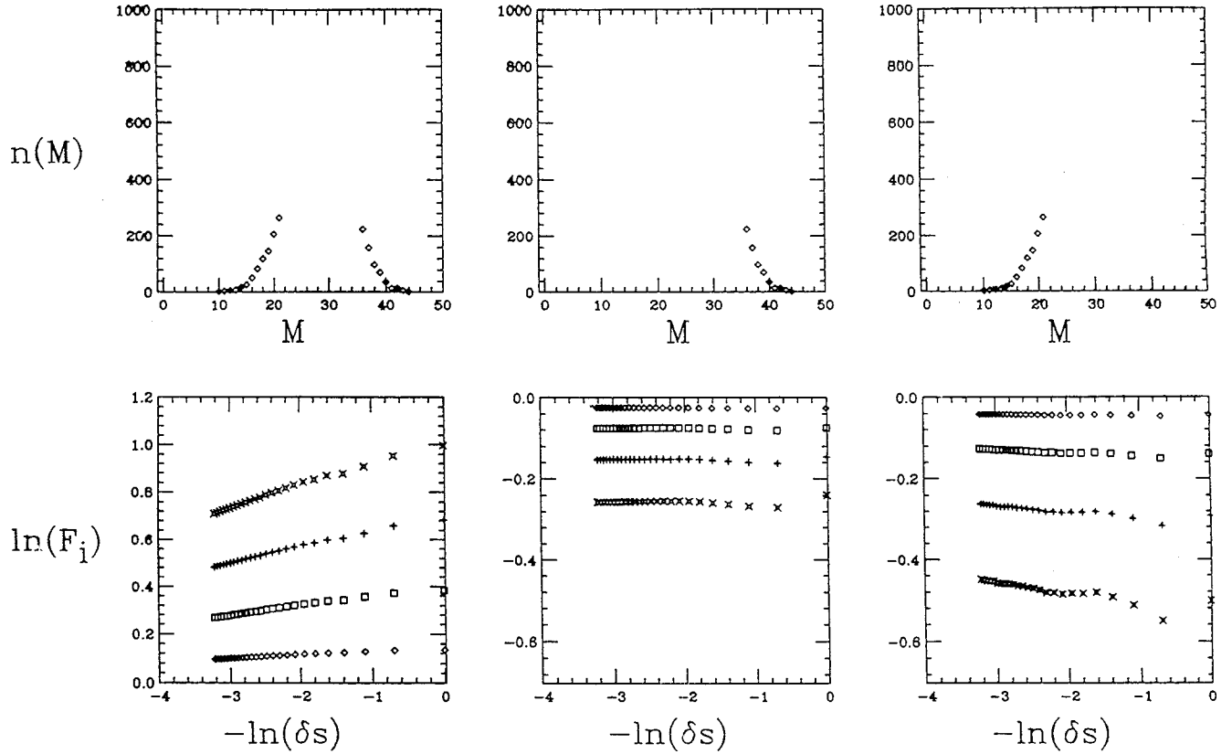
FIG. 8. Same as Fig. 7 but we show the effect of retaining only the liquidlike tail (right), the vaporlike tail (center), and when the two above mentioned are retained at the same time (left). It is clearly seen that for this last case not only intermittency is again present, but also it gets stronger.
