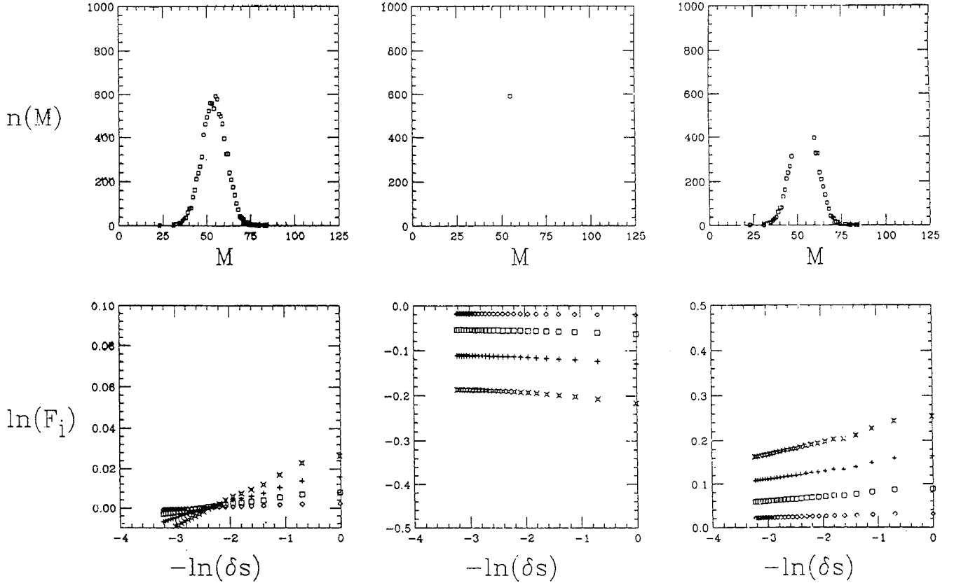
FIG. 10. Same as Fig. 7 but for percolation on a 5 \times 5 \times 5 lattice for a value of the bond parameter Q=0.24 .
