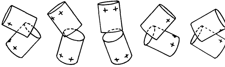
FIG. 5. Computer-drawn pictures of falling cat.
