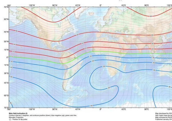
US/UK World Magnetic Model -- Epoch 2010.0 Main Field Inclination (I)
