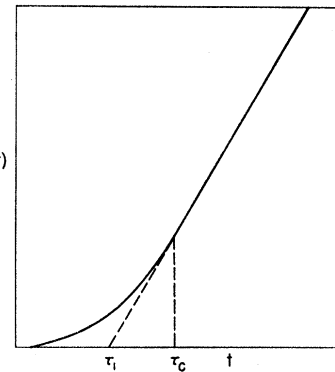
FIG. 4. The function \sigma(t) .
