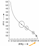
FIG. 89. The mass-radius relationship for white dwarfs (after Chandrasekhar, 1939). The masses are expressed in terms of the limiting mass M_0 and the radii in terms of a characteristic length l , which is given by 7.71\mu_e^{-1} \times 10^8 \text{ cm} \approx 3.86 \times 10^8 \text{ cm} .
