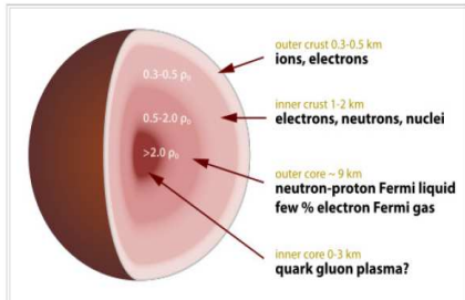
Cross-section of neutron star. Densities are in terms of \rho_0 the saturation nuclear matter density, where nucleons begin to touch.
