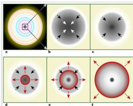
Within a massive, evolved star (a) the onion-layered shells of elements undergo fusion, forming a nickel-iron core (b) that reaches Chandrasekhar-mass and starts to collapse. The inner part of the core is compressed into neutrons (c), causing infalling material to bounce (d) and form an outward-propagating shock front (red). The shock starts to stall (e), but it is re-ignited by neutrino interaction. The surrounding material is blasted away (f), leaving only a degenerate remnant.
