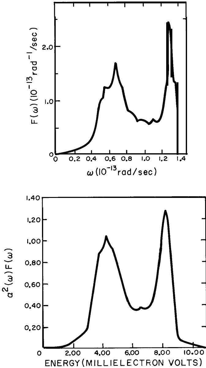
Comparison of \alpha^2 F(\omega) and F(\omega) for Pb (after McMillan and Rowell)
