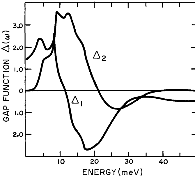
Real and imaginary parts of \Delta versus \omega for Pb.
