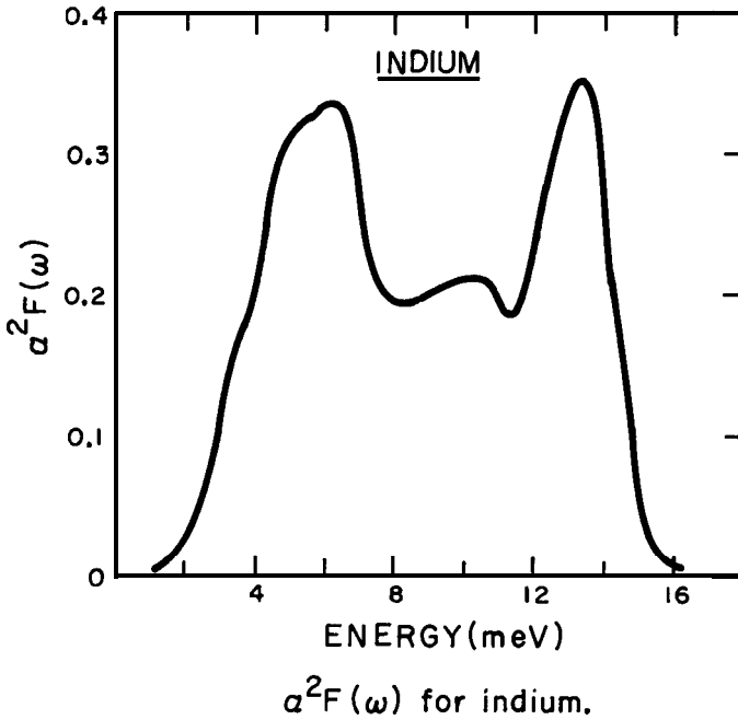
Fig. 6. \alpha^2 F for In (after McMillan and Rowell).
