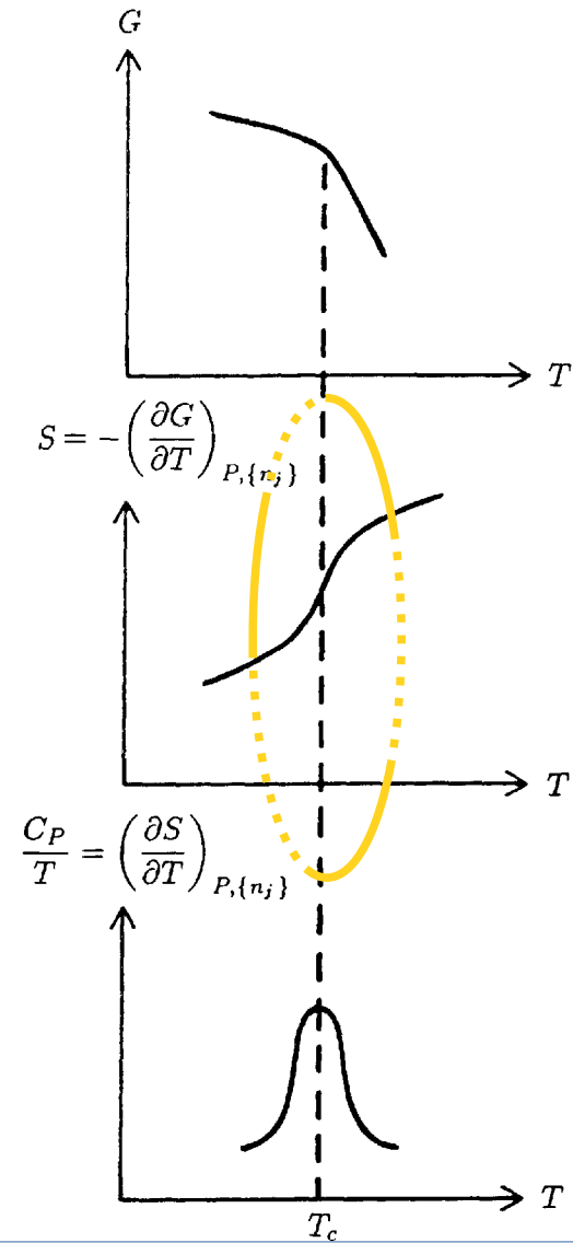
Fig. 3.3. Typical behavior for the Gibbs free energy at a continuous phase transition. The heat capacity can exhibit a peak at the transition.
