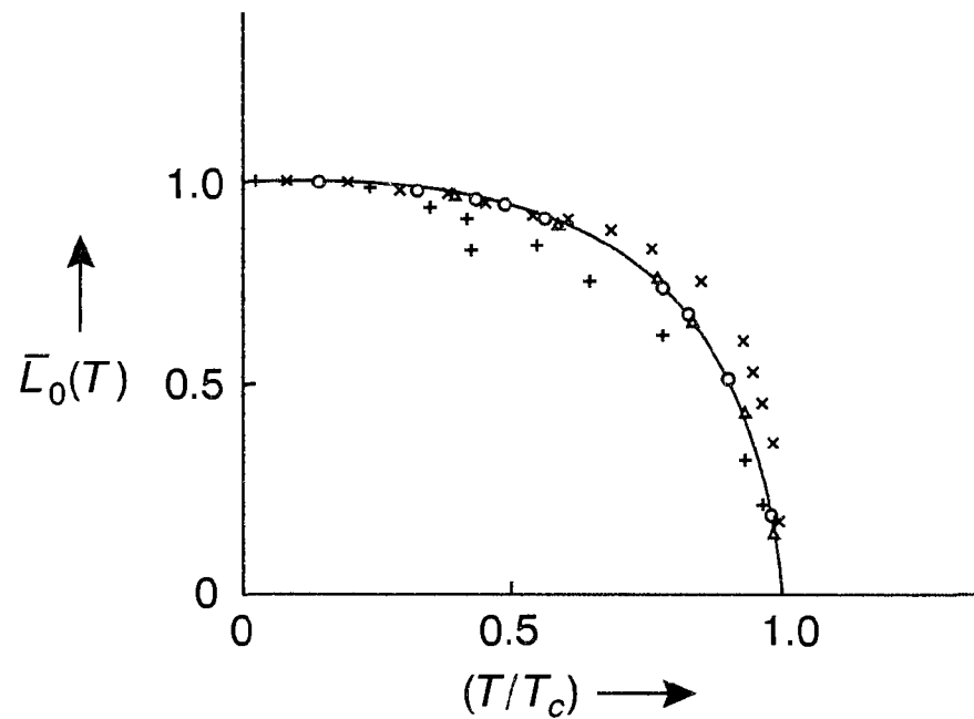
FIG. 11.7. The spontaneous magnetization of a Weiss ferromagnet as a function of temperature. The experimental points (after Becker) are for iron ( \times ), nickel (o), cobalt ( \Delta ) and magnetite (+).
