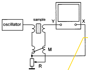
Fig. 1. Hartshorn bridge for determination of magnetic susceptibility
