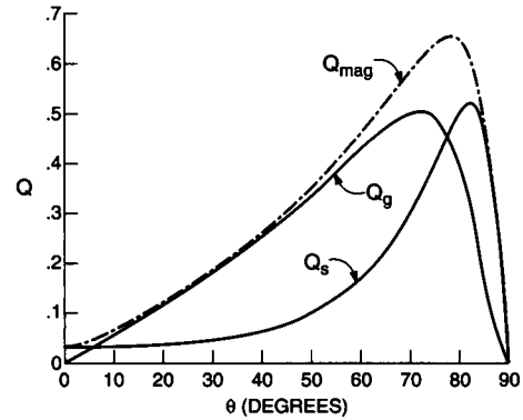
FIGURE 4 Values of the scattering force Q_s , gradient force Q_g , and magnitude of the total force Q_{\text{mag}} for a single ray hitting a dielectric sphere of index of refraction n = 1.2 at an angle \theta .
