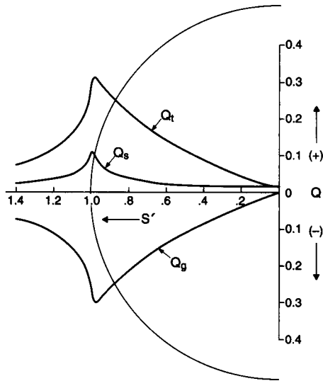
FIGURE 7 Plot of the gradient force, scattering force, and total force Q_g , Q_s , and Q_t as a function of the distance S' of trap focus from the origin along the -Y axis for a circularly polarized trapping beam uniformly filling the aperture and a sphere of index of refraction n = 1.2 .
