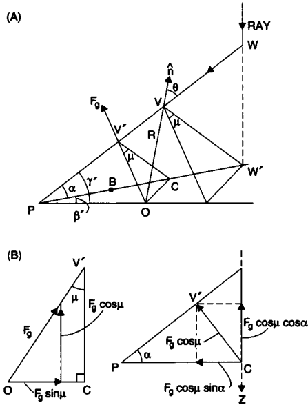
FIGURE 9 Another view of Fig. 8A containing the angle \mu between the plane of incidence POV' and the vertical plane WW'P for resolving force components along the coordinate axis.
