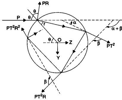
FIGURE 3 Geometry for calculating the force due to the scattering of a single incident ray of power P by a dielectric sphere, showing the reflected ray PR and infinite set of refracted rays PT^2R^n .
