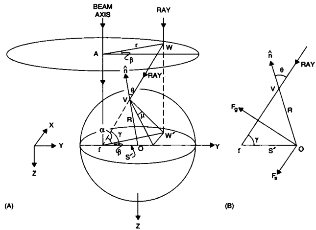
FIGURE 6 (A) Trap geometry with the beam focus f located transversely along the -Y axis at a distance S' from the origin. (B) Geometry of the plane of incidence showing the directions of the gradient and scattering forces F_g and F_s for the input ray.
