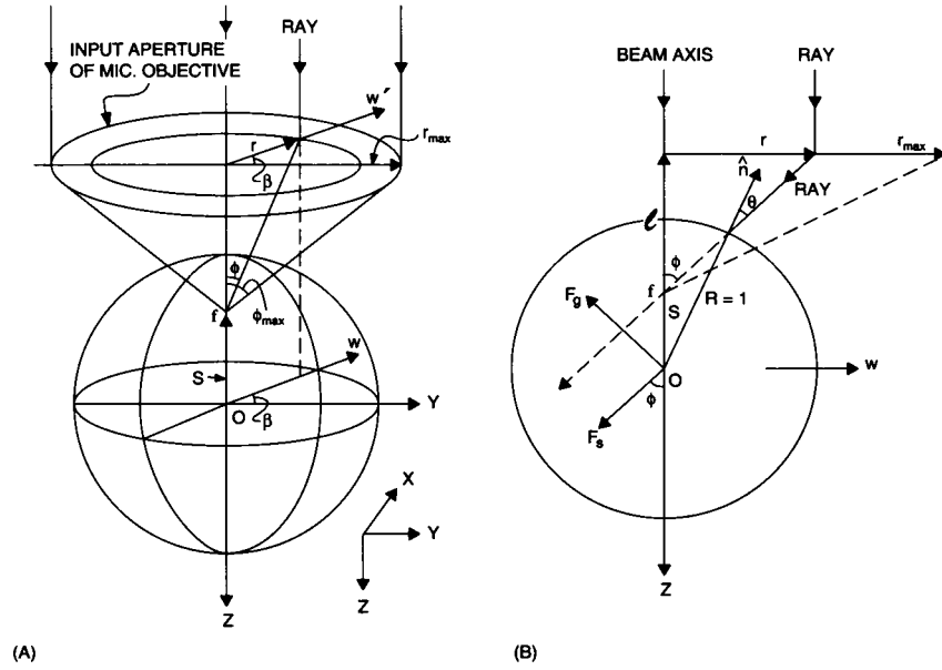
FIGURE 2 (A) Single beam gradient force trap in the ray optics model with beam focus f located along the Z axis of the sphere. (B) Geometry of an incident ray giving rise to gradient and scattering force contributions F_g and F_s .
