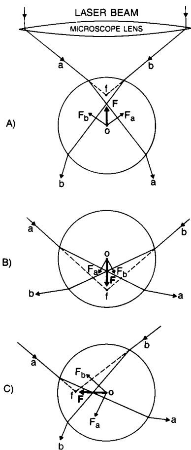
FIGURE 1 Qualitative view of the trapping of dielectric spheres. The refraction of a typical pair of rays a and b of the trapping beam gives forces F_a and F_b , whose vector sum F is always restoring for axial and transverse displacements of the sphere from the trap focus f .
