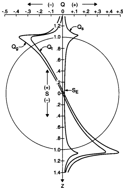
FIGURE 5 Values of the scattering force, gradient force, and total force Q_s , Q_g , and Q_t exerted on a sphere of index of refraction n = 1.2 by a trap with a uniformly filled input aperture which is focused along the Z axis at positions +s above and -s below the center of the sphere.
