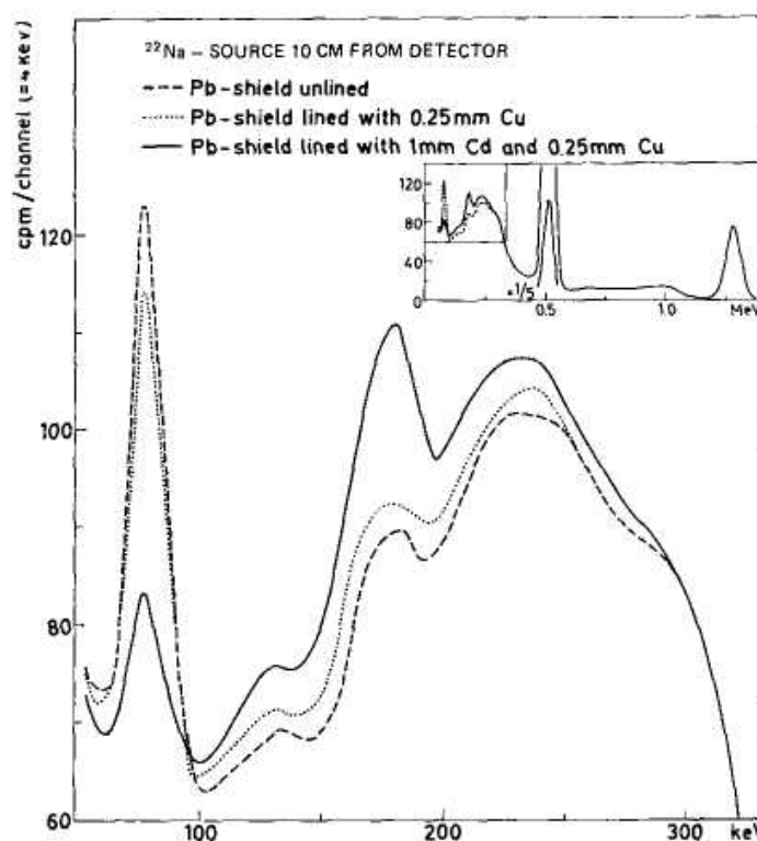
Figure 20.5 A plot of the low-energy portion of the ^{22}\text{Na} gamma-ray spectrum (indicated on the insert) as recorded by a 7.62\text{ cm} \times 7.62\text{ cm} \text{NaI(Tl)} scintillator. The effects of different shield liners on the fluorescent X-ray and backscatter peaks are illustrated. (From Stenberg and Olsson. 9 )
