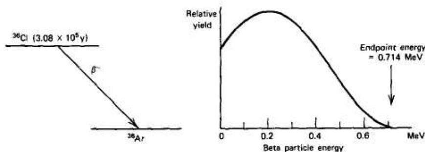
Figure 1.1 The decay scheme of ^{36}\text{Cl} and the resulting beta particle energy distribution.
