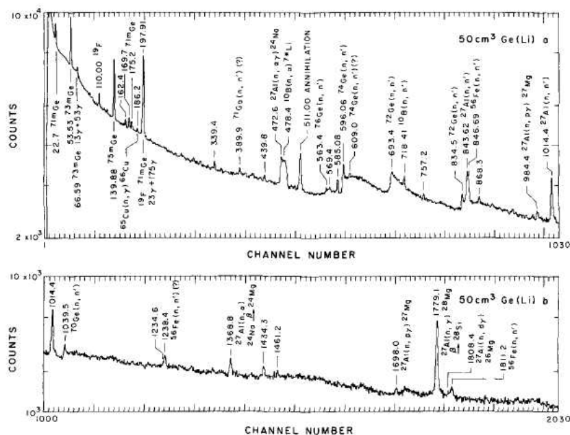
Figure 12.34 Prompt pulse height spectrum produced by fast neutron irradiation of a 50 cm 3 Ge(Li) detector. (From Bunting and Kraushaar. 102 )
