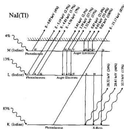
Figure 10.21 Representation of the possible origins of electrons and photons following the photoelectric absorption of an incident X-ray or gamma ray with energy E that is above the K -shell binding energy of 33.17 keV. (From Rooney and Valentine. 27 )
