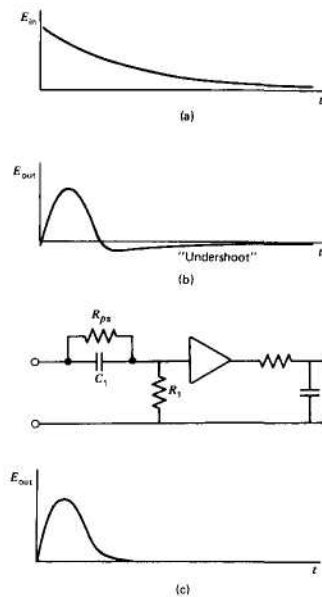
Figure 16.15 Application of pole-zero cancellation to eliminate the undershoot ( b ) normally generated by a CR - RC shaping network for an input step with finite decay time. By adding an appropriate resistance R to the differentiator stage, a waveform without undershoot ( c ) can be obtained.
