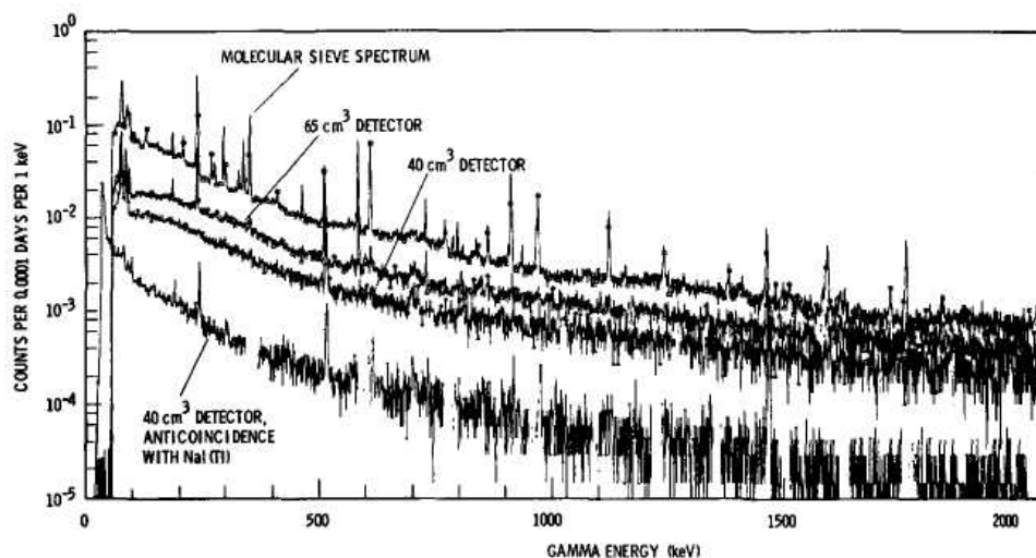
Figure 20.9 The bottom spectrum shows the degree to which background in a 40-cm 3 germanium detector may be suppressed through the use of an annular NaI(Tl) scintillator in anticoincidence. A comparison of the two middle spectra illustrates the increase in background with detector active volume. The top curve shows the recorded spectrum using a sample of molecular sieve (a part of some germanium vacuum systems) as a source of natural background radiation. (From Kaye et al. 10 )
