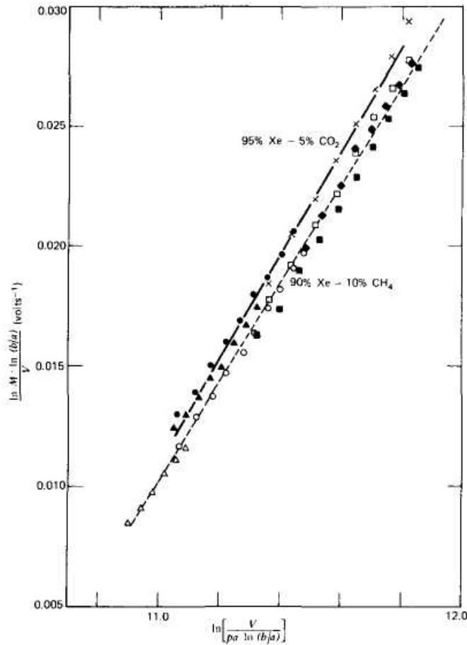
Figure 6.11 A Diethorn plot of the same data shown in Fig. 6.10. As predicted by Eq. (6.8), a graph of [\ln M \times \ln(b/a)/V] versus \ln[V/p \ln(b/a)] for all counters using the same gas closely matches a straight line with slope of (\ln 2/\Delta V) and intercept (-\ln 2)(\ln K)/\Delta V . (Prom Hendricks. 49 )
