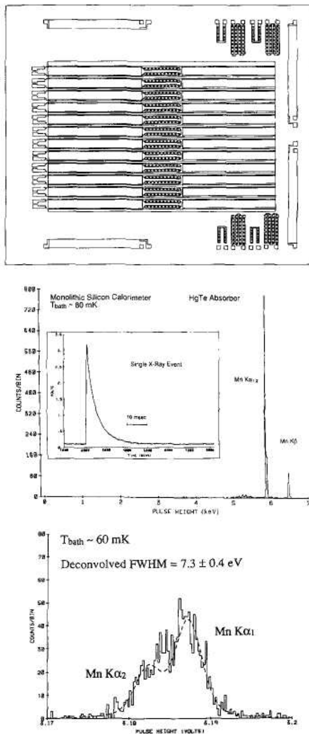
Figure 19.7 Array of 12 microcalorimeter elements, each 0.25 mm X 1.0 mm X 15 \mu\text{m} thick. The corresponding energy spectrum from a ^{55}\text{Fe} source is shown in both a normal and expanded scale. A typical pulse profile is shown in the insert. (From McCammon et al. 46 )
