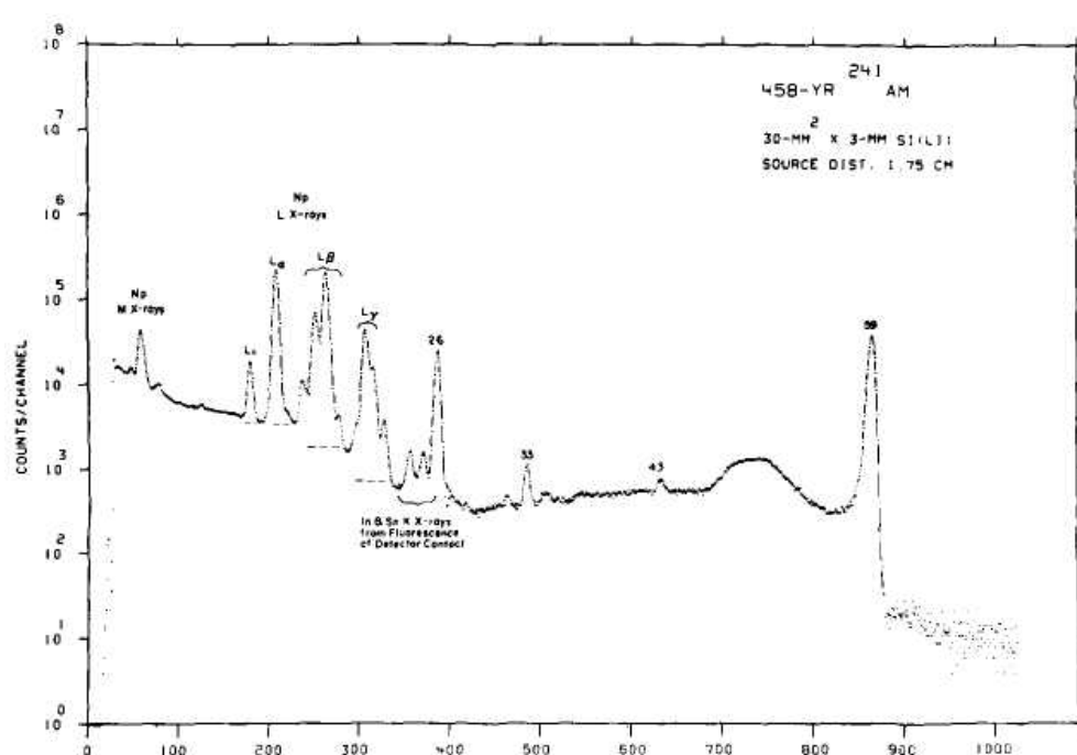
Figure 13.13 Photon spectrum from ^{241}\text{Am} obtained using a 30 mm 2 X 3 mm Si(Li) detector. (From Gehrke and Lokken. 29 )
