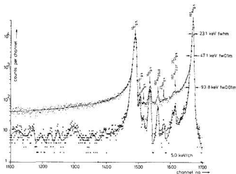
Figure 13.6 Comparison of pulse height spectra from a Si(Li) detector with (X) and without (•) rejection of pulses with rise times greater than 70 ns. The source was a proton beam scattered from several target nuclides. (From Lindstrom and Lisdat. 9 )
