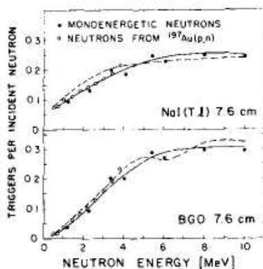
Figure 10.30 The prompt pulse response to fast neutrons in 7.6 cm \times 7.6 cm scintillation detectors of NaI(Tl) and BGO. (From Hausser et al. 46 )
