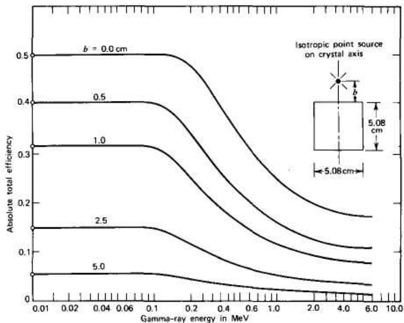
Figure 10.22 The absolute total efficiency calculated for a 5.08 cm \times 5.08 cm solid cylindrical NaI(Tl) scintillator. Different values of the source location are shown. (From Snyder. 28 )
