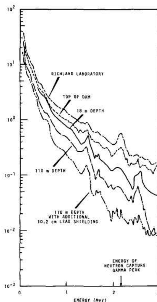
Figure 20.6 The background spectra from a 7.62 cm \times 7.62 cm NaI(Tl) scintillator within a paraffin and 10.2 cm thick lead shield. The indicated locations are at different depths within the massive concrete structure of Grand Coulee Dam. The purpose of the paraffin was to indicate the importance of the neutron component by the relative prominence of the hydrogen capture gamma-ray peak at 2.22 MeV. (From Kaye et al. 19 )
