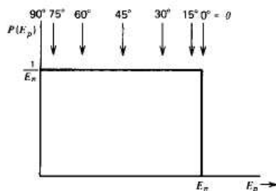
Figure 15.14 Energy distribution of recoil protons E produced by monoenergetic neutrons. Recoil energies are indicated for various values of the recoil emission angle \theta as given by Eq. (15.3). For scattering from hydrogen, E_p is equivalent to E_R in Eqs. (15.1) through (15.7).
