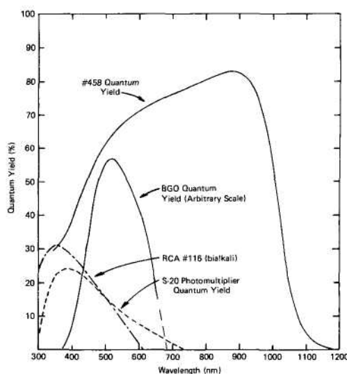
Figure 9.15 A comparison of the quantum efficiency of a silicon photodiode (labeled #458) with representative bialkali and S-20 photo-cathode quantum efficiencies. The emission spectrum from a BGO scintillator is shown for reference. (From Groom. 63 )
