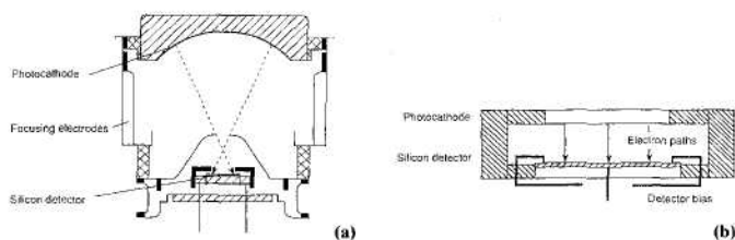
Figure 9.21 Elements of hybrid photomultiplier tubes. Part (a) shows the electrostatic focusing arrangement, while part (b) shows a proximity-focused configuration. (From Basa, et al. 78 )
