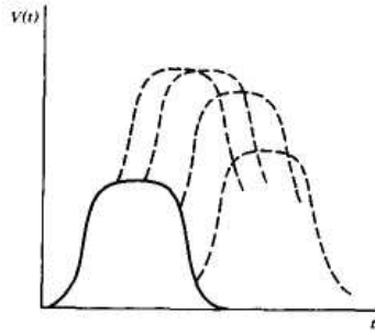
Figure 17.18 Peak pile-up in which two closely spaced signal pulses combine to form one distorted pulse. Several different cases are sketched with increasing overlap between the first and second pulse.
