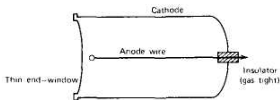
Figure 7.6 A cross section of a typical end-window Geiger tube.
