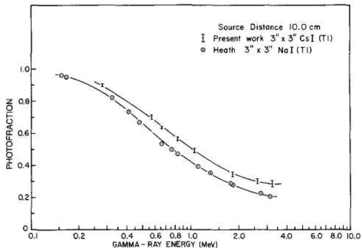
Figure 10.27 Experimental photofractions of 7.62 cm x 7.62 cm cylindrical crystals of CsI(Tl) and NaI(Tl). (From Irfan and Prasad. 39 )
