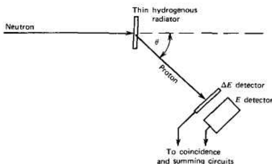
Figure 15.22 A proton recoil telescope.
