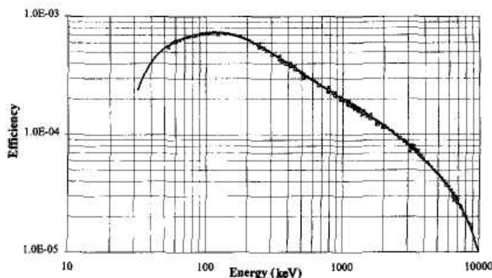
Figure 12.31 The points shown are measured full-energy peak efficiency values for a 25% relative efficiency n-type germanium detector. The cryostat had a 0.5 mm thick aluminum entrance window. The points at lower energies were obtained using standard radioisotope calibration sources, whereas neutron-induced capture gamma rays provided the upper energy values. The solid line is a 9-parameter analytical fit to all the points using a function of the form given in Eq. (12.32). (From Kis et al. 89 )
