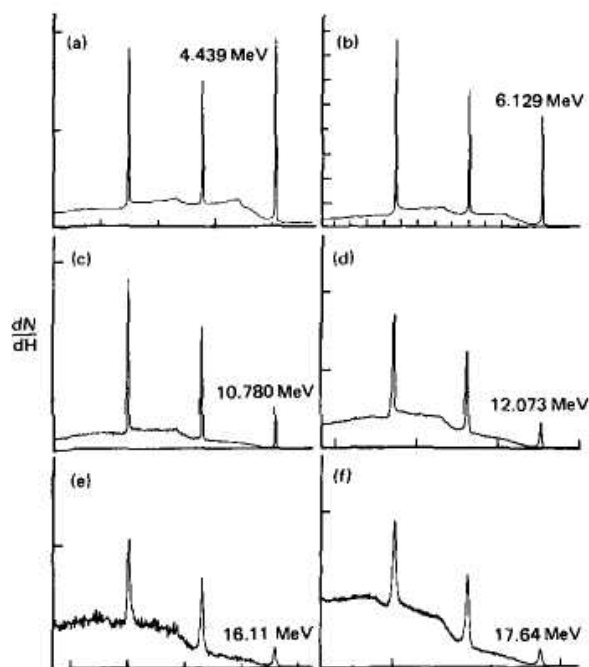
Figure 12.17 The relative intensity of the full-energy, single escape, and double escape peaks for a 100\text{ cm}^3 Ge(Li) detector for gamma-ray energies from 4.439 to 17.64 MeV. (From Berg et al. 45 )
