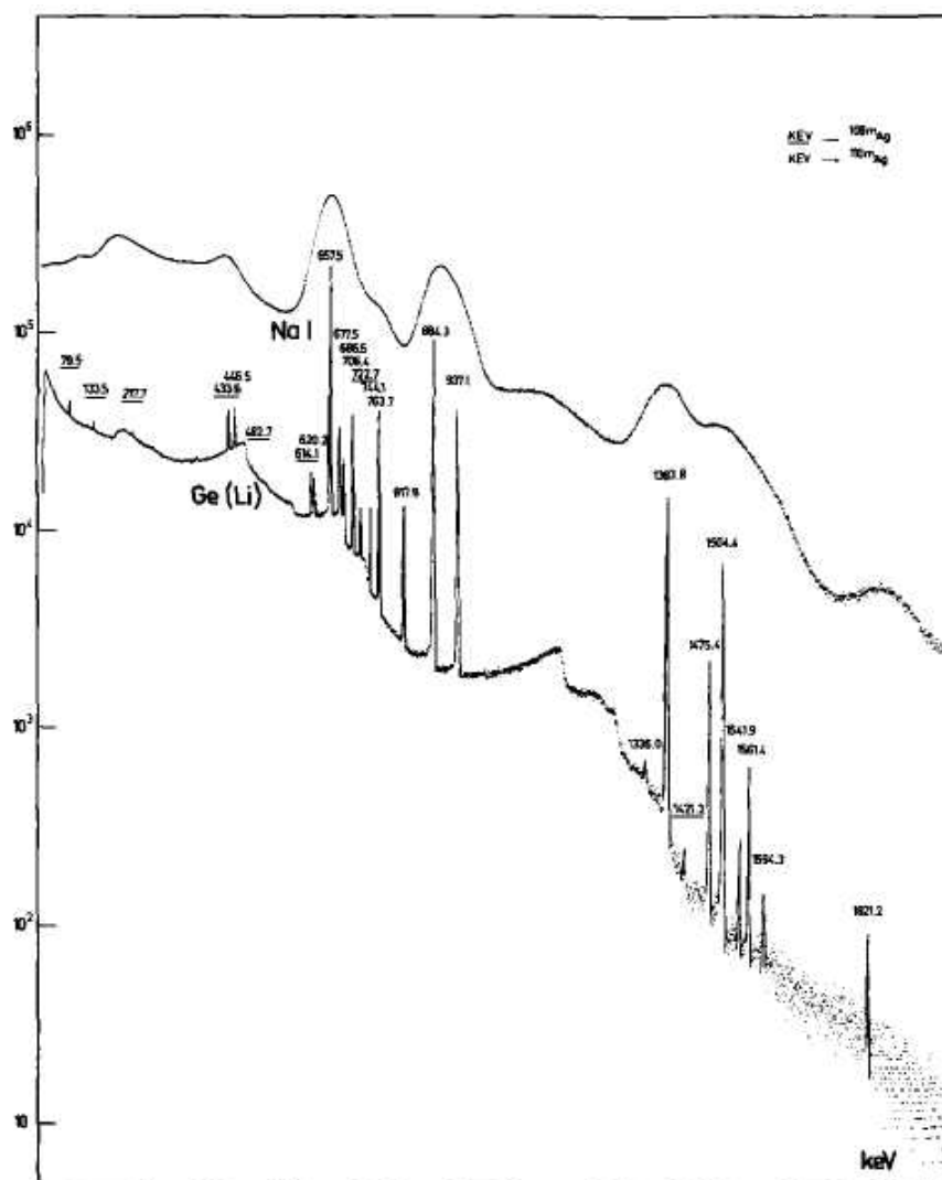
Figure 12.7 Comparative pulse height spectra recorded using a sodium iodide scintillator and a \text{Ge(Li)} detector. The source was gamma radiation from the decay of ^{108m}\text{Ag} and ^{110m}\text{Ag} . Energies of peaks are labeled in keV. (From Philippot. 13 )
