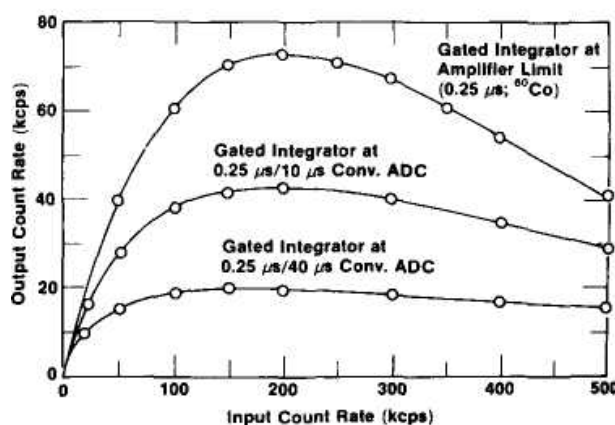
Figure 17.26 An example of the throughput of a pulse-processing system at high input rates. In this case, a gated integrator allows the use of a short (0.25 \mu s) Gaussian shaping time. The top curve is for the amplifier alone. The remaining plots show the additional losses due to the conversion time of the ADC of the multichannel analyzer used to record the pulses. (From Britton et al. 9 )
