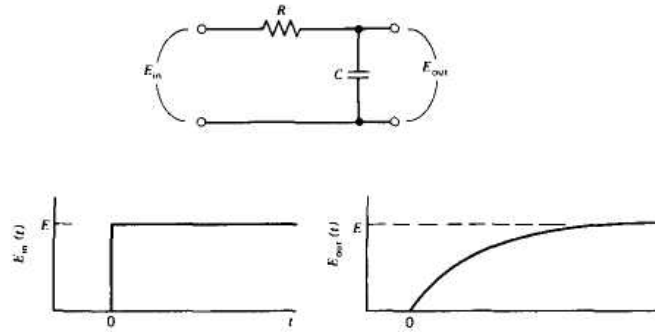
Figure 16.10 A low-pass RC filter or integrator network. The response to a step function input is illustrated.
