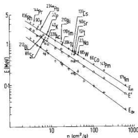
Figure 2.16 Beta particle absorption coefficient n in aluminum as a function of the endpoint energy E_m , average energy E_{av} , and E' = 0.5 (E_m + E_{av}) of different beta emitters. (From Baltakmens. 26 )
