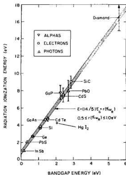
Figure 13.21 The average energy required to form one electron-hole pair (e) versus bandgap energy for a number of semiconductor materials. (From Klein. 45 )
