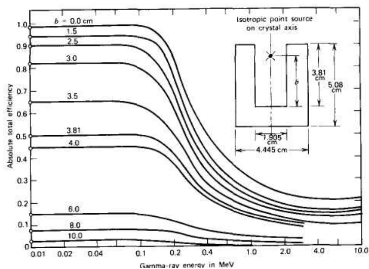
Figure 10.23 The absolute total efficiency calculated for a point gamma-ray source and a NaI(Tl) well-type scintillator with the dimensions shown. The parameter b is the source height above the well bottom. (From Snyder. 28 )
