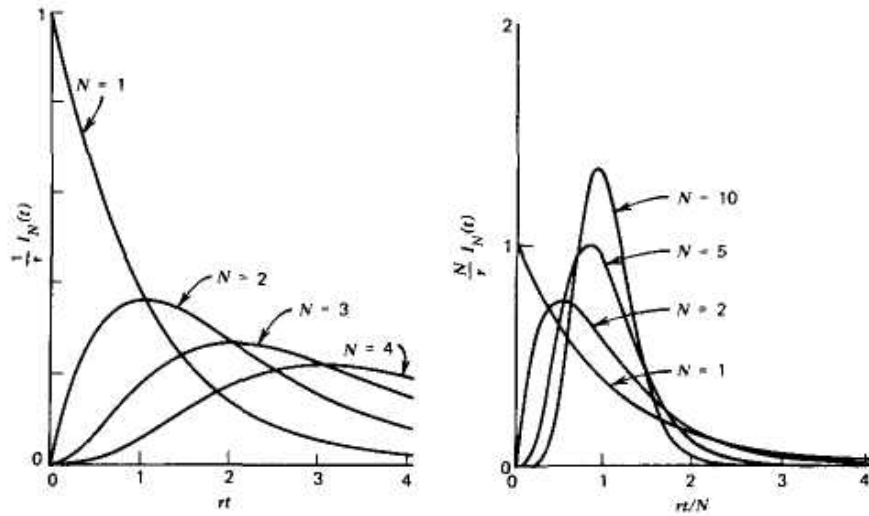
Figure 3.15 Graphical representation of the scaled interval distribution I_N(t) . (a) Four distributions for scaling factors of 1, 2, 3 and 4. (b) Interval distributions for N=1 through N=10 normalized to the same average interval N/r .
