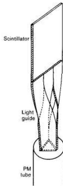
Figure 8.16 A strip light guide can be used to couple the edge of a large, flat scintillator to a PM tube.
