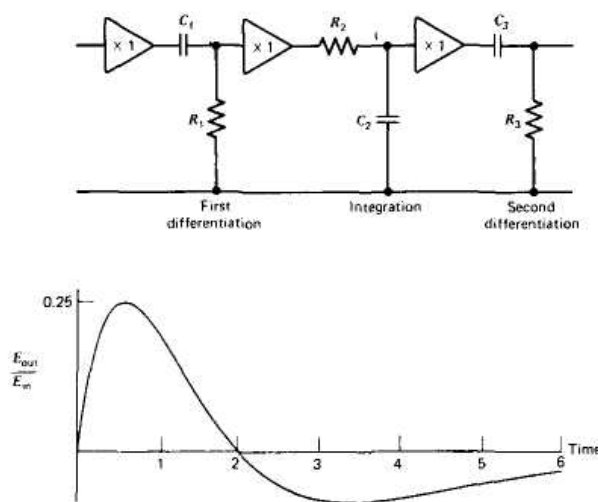
Figure 16.19 The CR - RC - CR network and its output waveform for a step input when all three time constants are equal. Units of the time scale are in values of this time constant.
