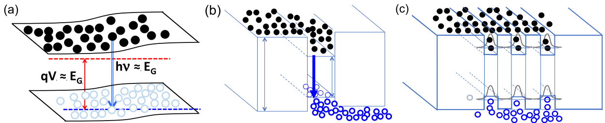
Fig. 10. Schematics of real-space band diagram and carrier diffusion in forward biased, from (a) p-n homojunction, (b) p-n double heterostructure, (c) p-n multi-quantum well structure.
