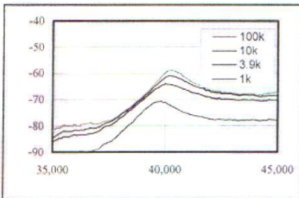
Sensitivity change with load impedance
