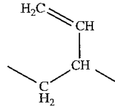
vinyl
