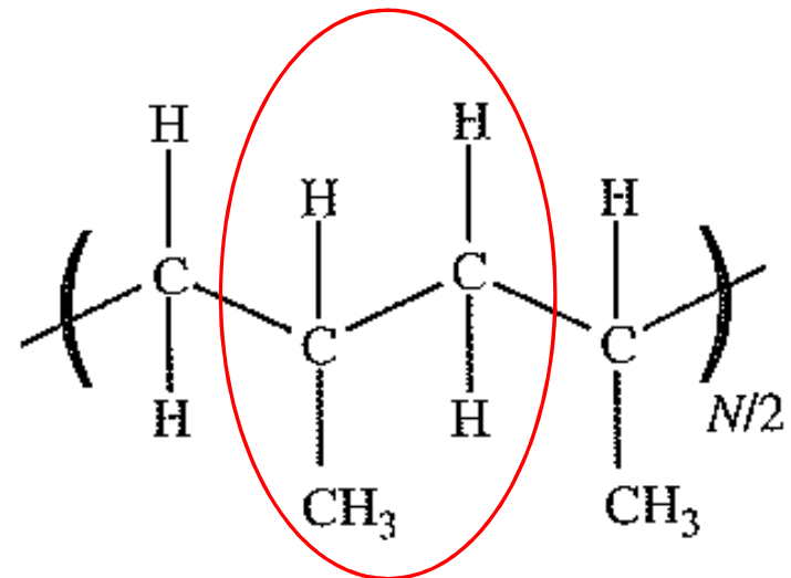
Head-to-tail polypropylene
