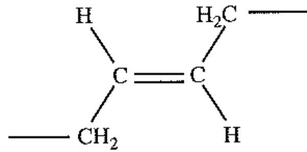
trans
