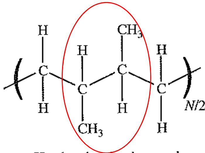
Head-to-head polypropylene
