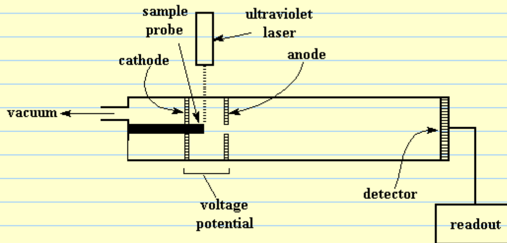
A simplified diagram of a MALDI apparatus (After Creel, H., Trends in Polym. Sci. , 1993, 1(11), 336-342.)
